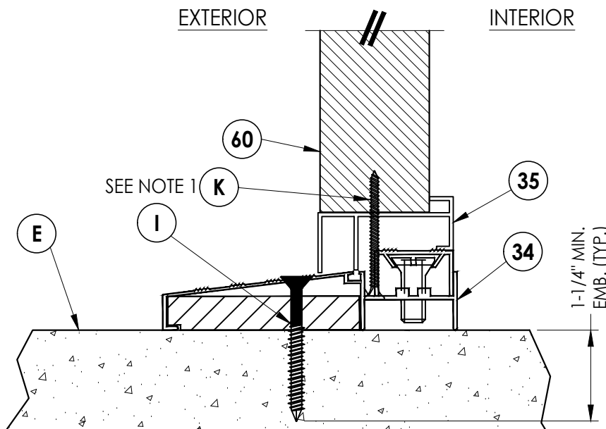
3 VERTICAL CROSS SECTION 8 Inswing configuration
