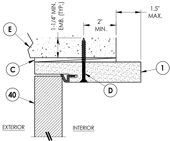
2 VERTICAL CROSS SECTION Shown Direct to Masonry Outswing only w/ 6-9/16" jamb
