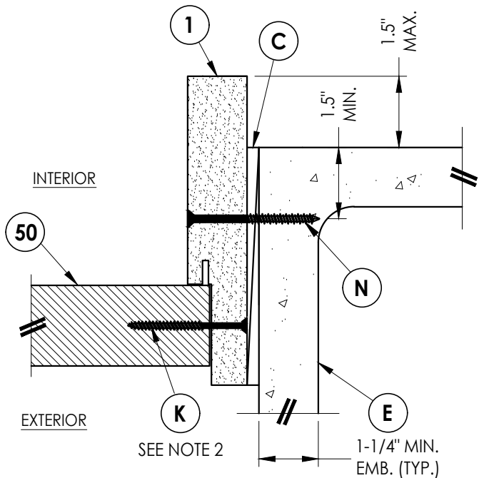
1 HORIZONTAL CROSS SECTION Shown Direct to Masonry Outswing only w/ 6-9/16" jamb
