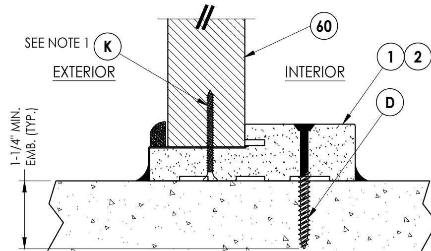
5 VERTICAL CROSS SECTION 8 Inswing configuration
