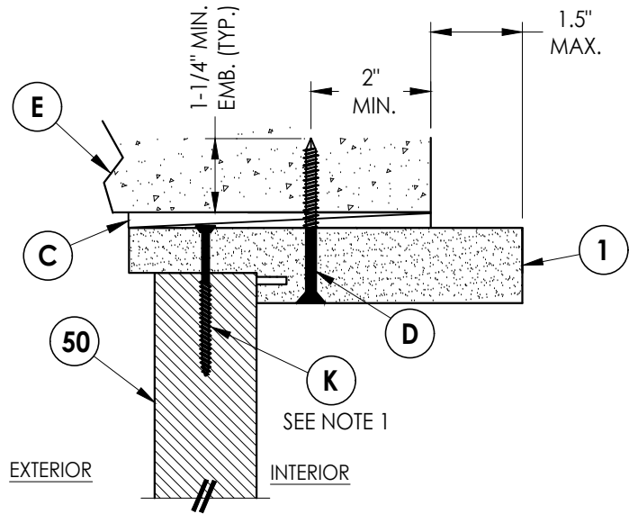
3 VERTICAL CROSS SECTION Shown Direct to Masonry Outswing only w/ 6-9/16" jamb
